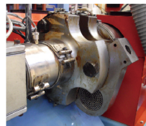
Lever type manual screen changer
