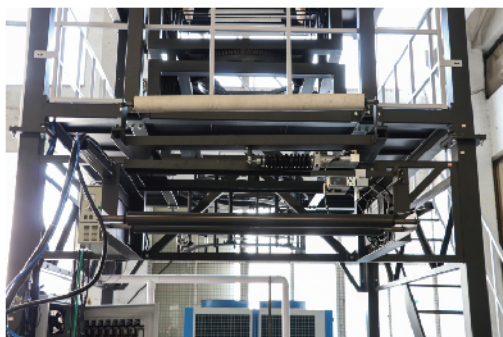
Central position control system
